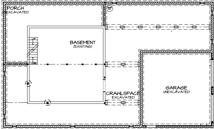
FOUNDATION PLAN A-3
